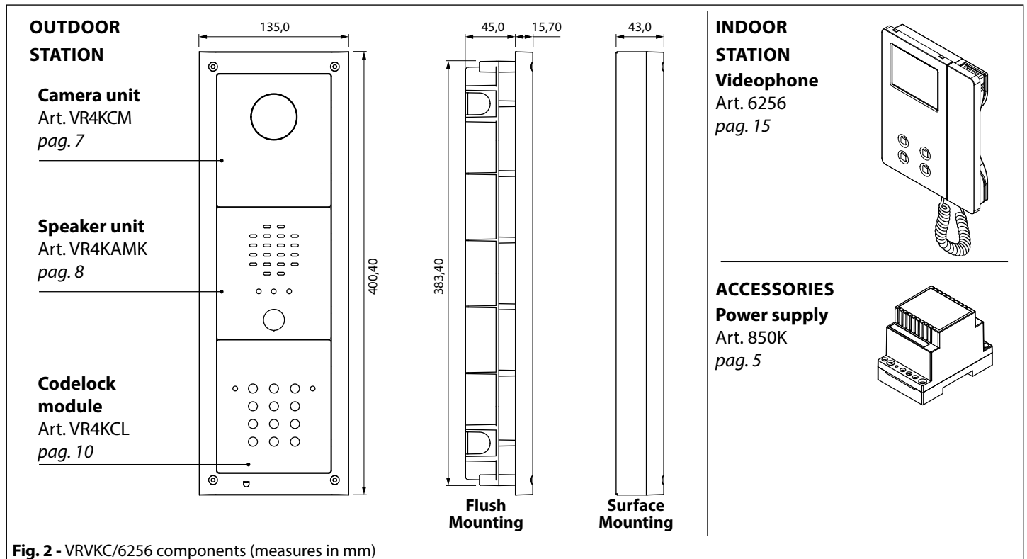
Fig. 2 - VRVKC/6256 components (measures in mm)
