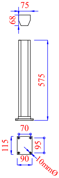
401028 Support Post
